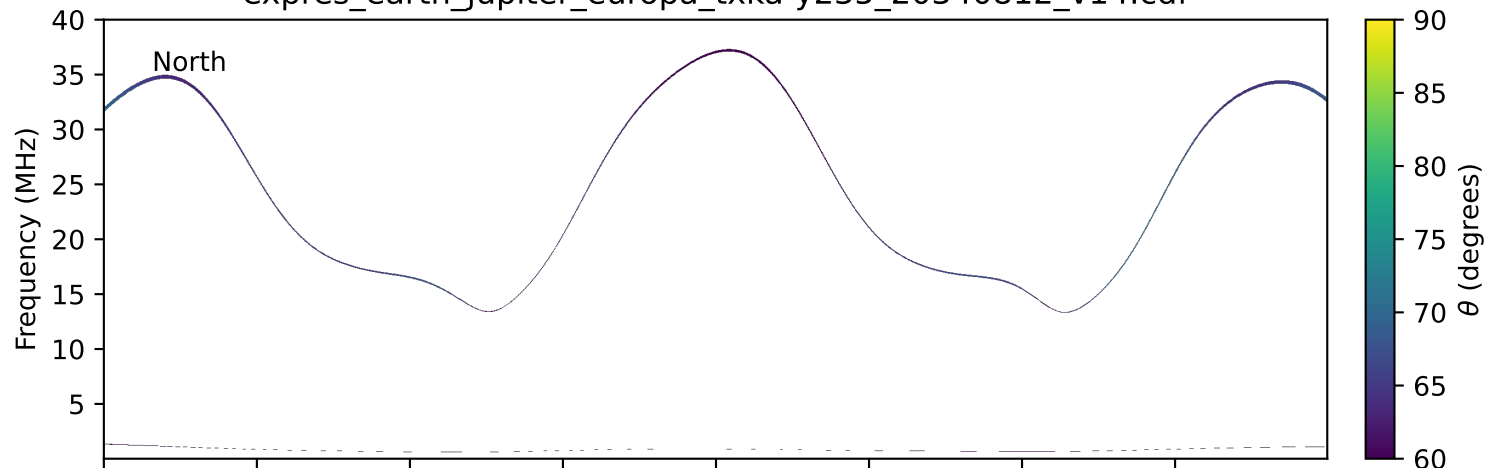
expres_earth_jupiter_europa_txka-y235_20340812_v14.cdf
