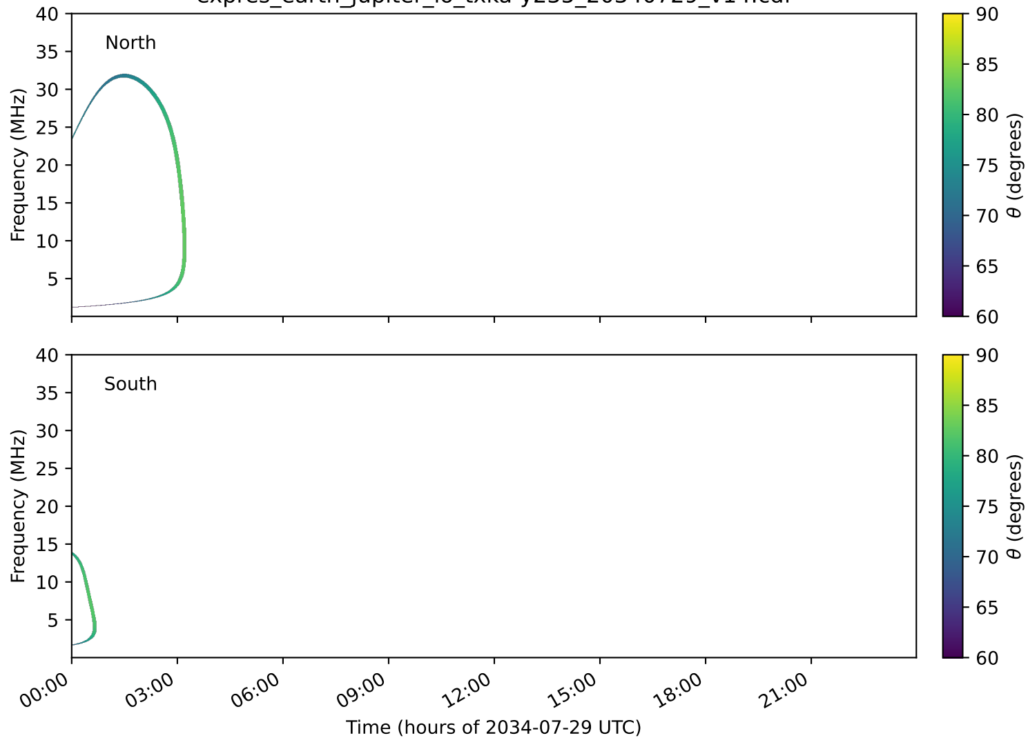
expres_earth_jupiter_io_txka-y235_20340729_v14.cdf
