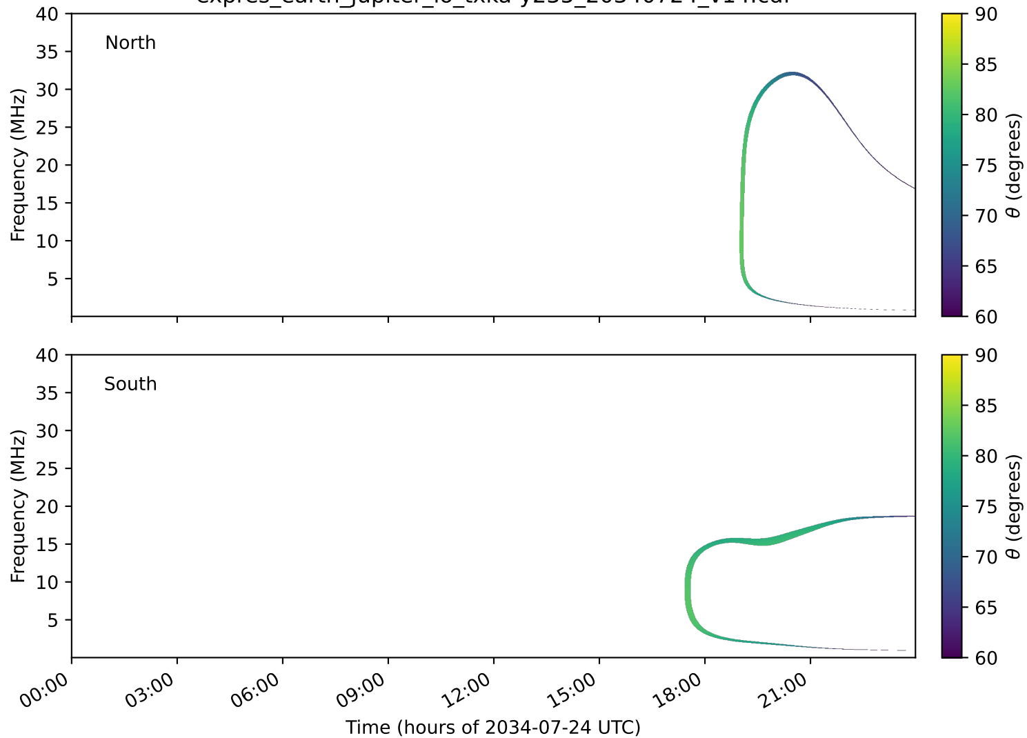
expres_earth_jupiter_io_txka-y235_20340724_v14.cdf
