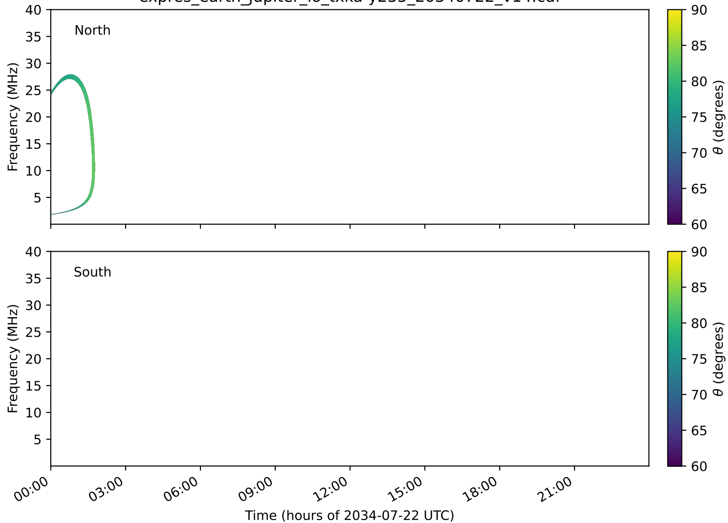
expres_earth_jupiter_io_txka-y235_20340722_v14.cdf
