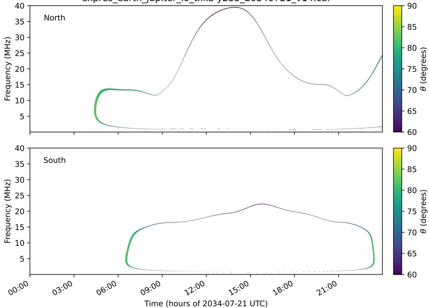
expres_earth_jupiter_io_txka-y235_20340721_v14.cdf
