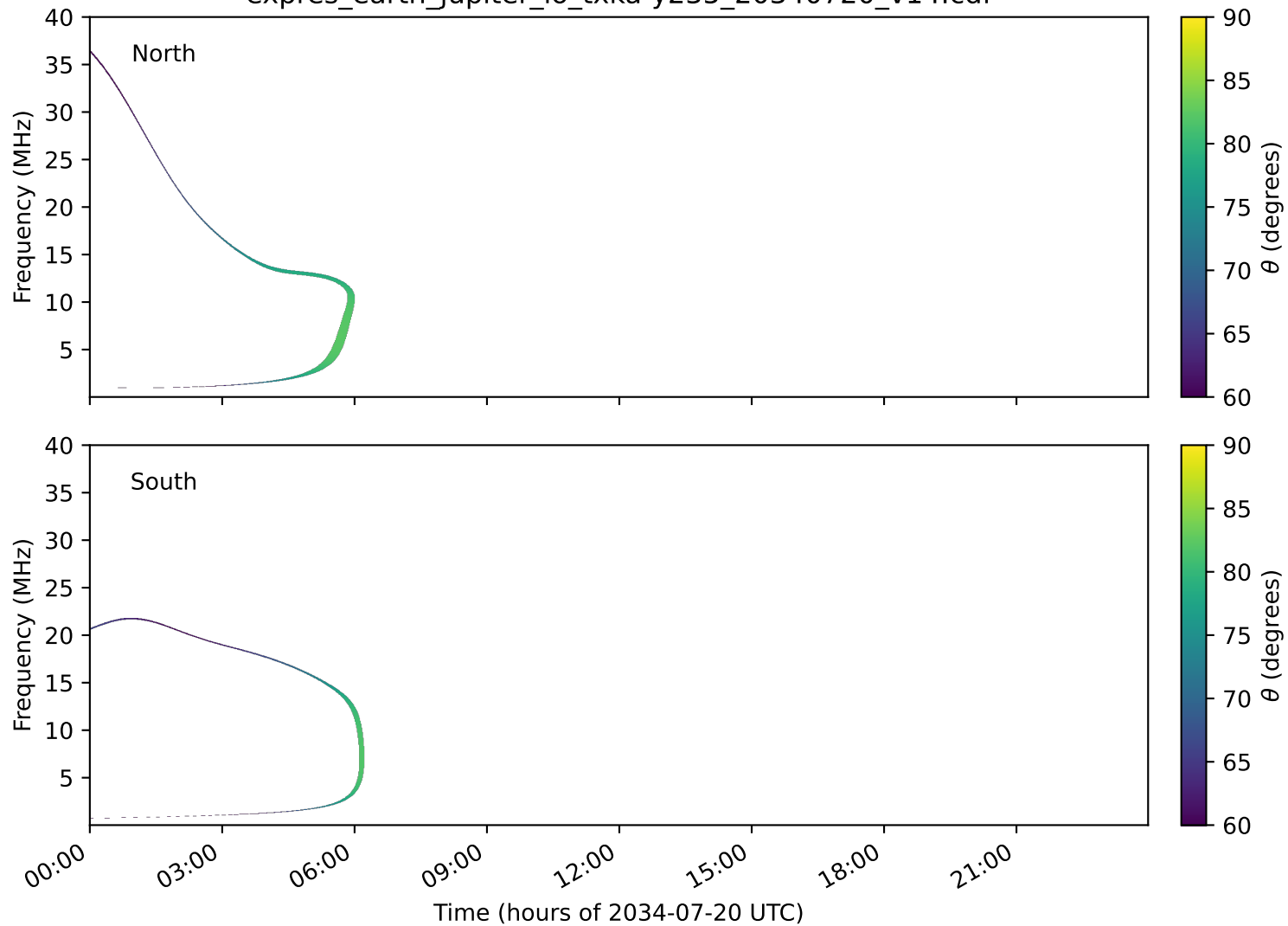
expres_earth_jupiter_io_txka-y235_20340720_v14.cdf
