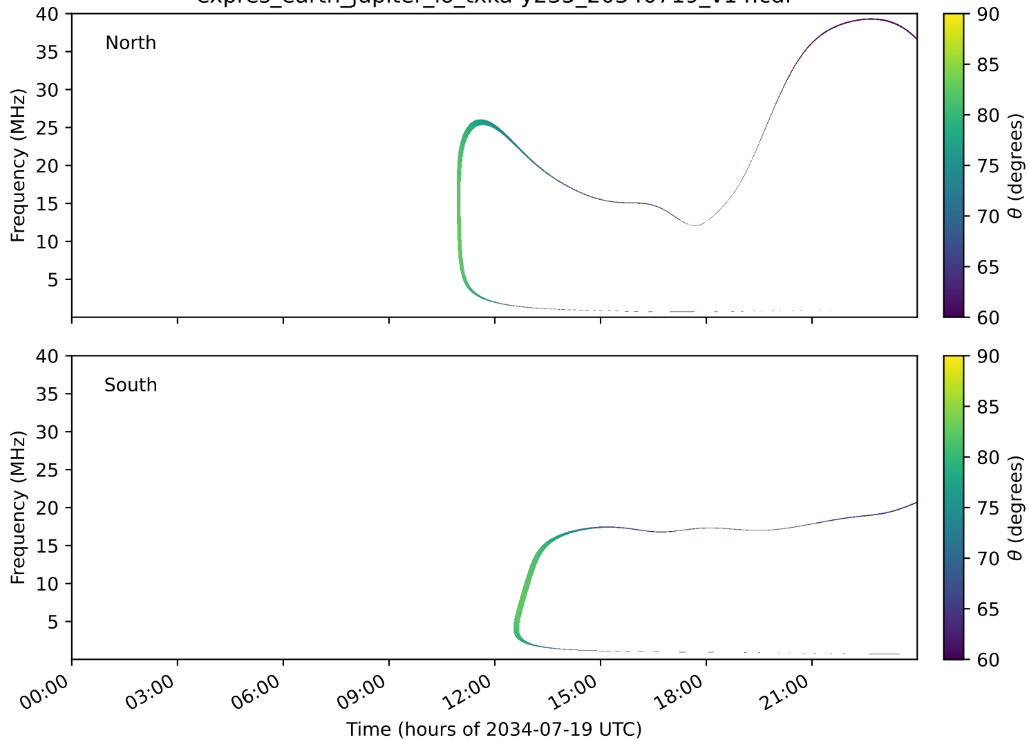
expres_earth_jupiter_io_txka-y235_20340719_v14.cdf
