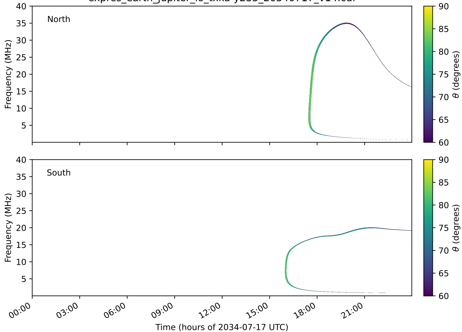
expres_earth_jupiter_io_txka-y235_20340717_v14.cdf
