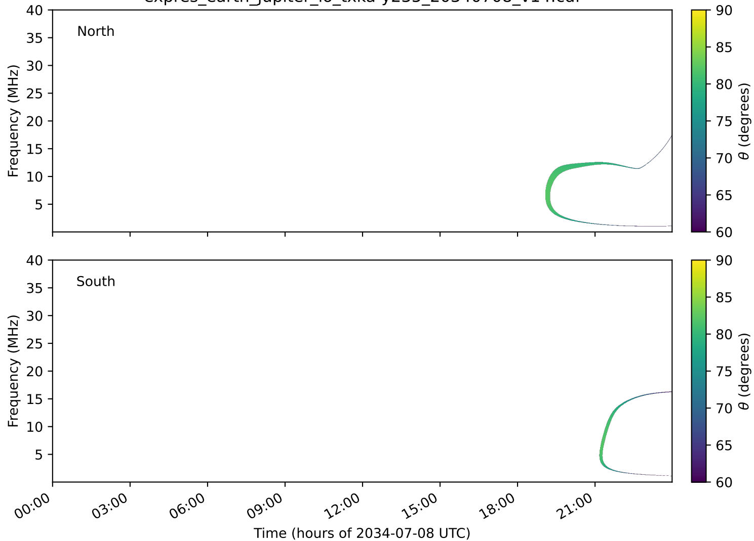
expres_earth_jupiter_io_txka-y235_20340708_v14.cdf
