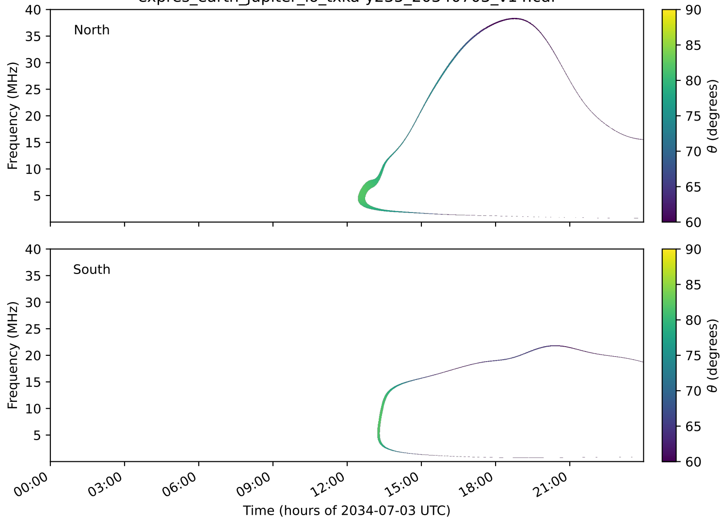
expres_earth_jupiter_io_txka-y235_20340703_v14.cdf
