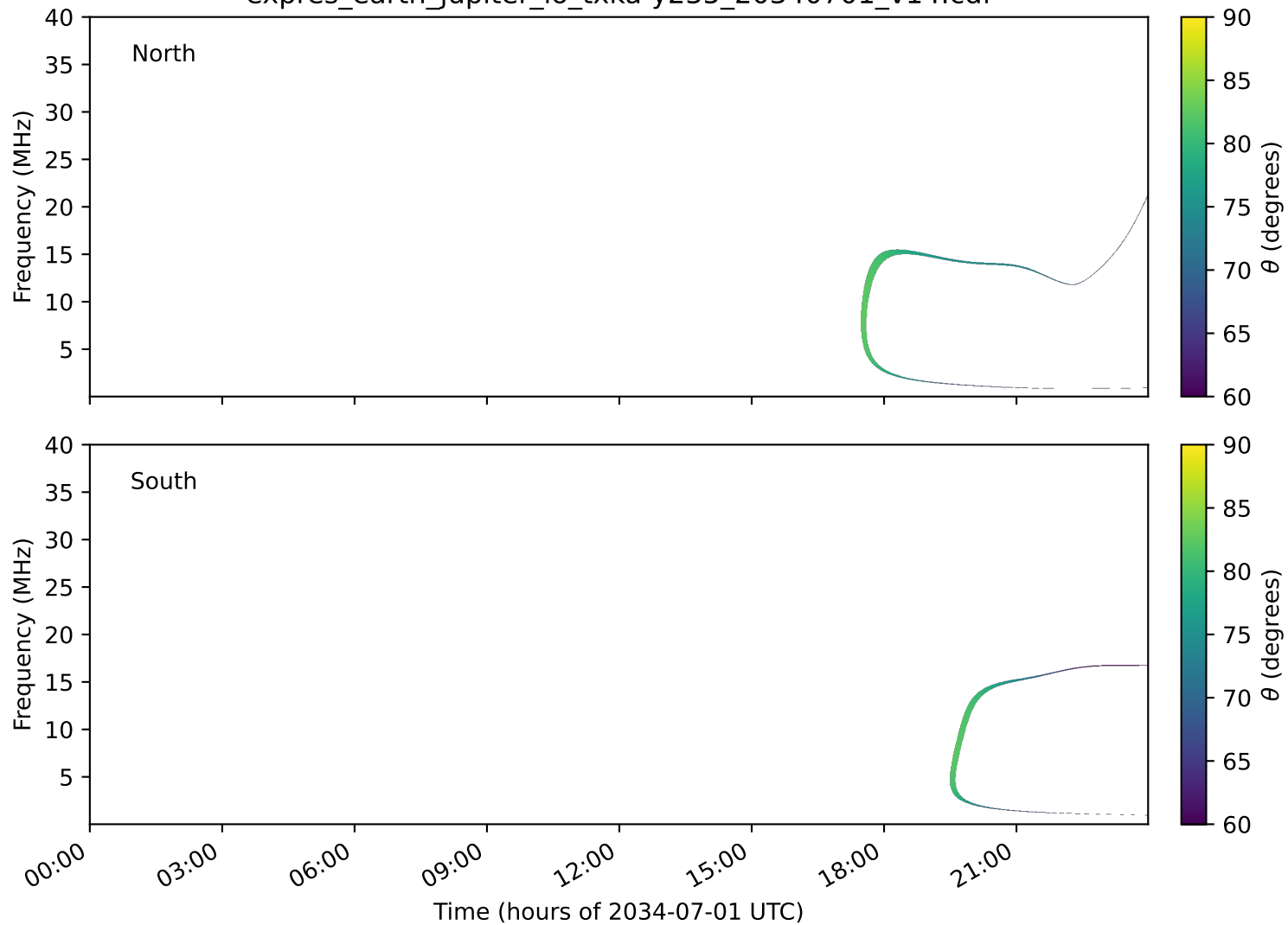
expres_earth_jupiter_io_txka-y235_20340701_v14.cdf
