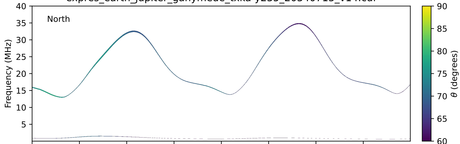
expres_earth_jupiter_ganymede_txka-y235_20340713_v14.cdf
