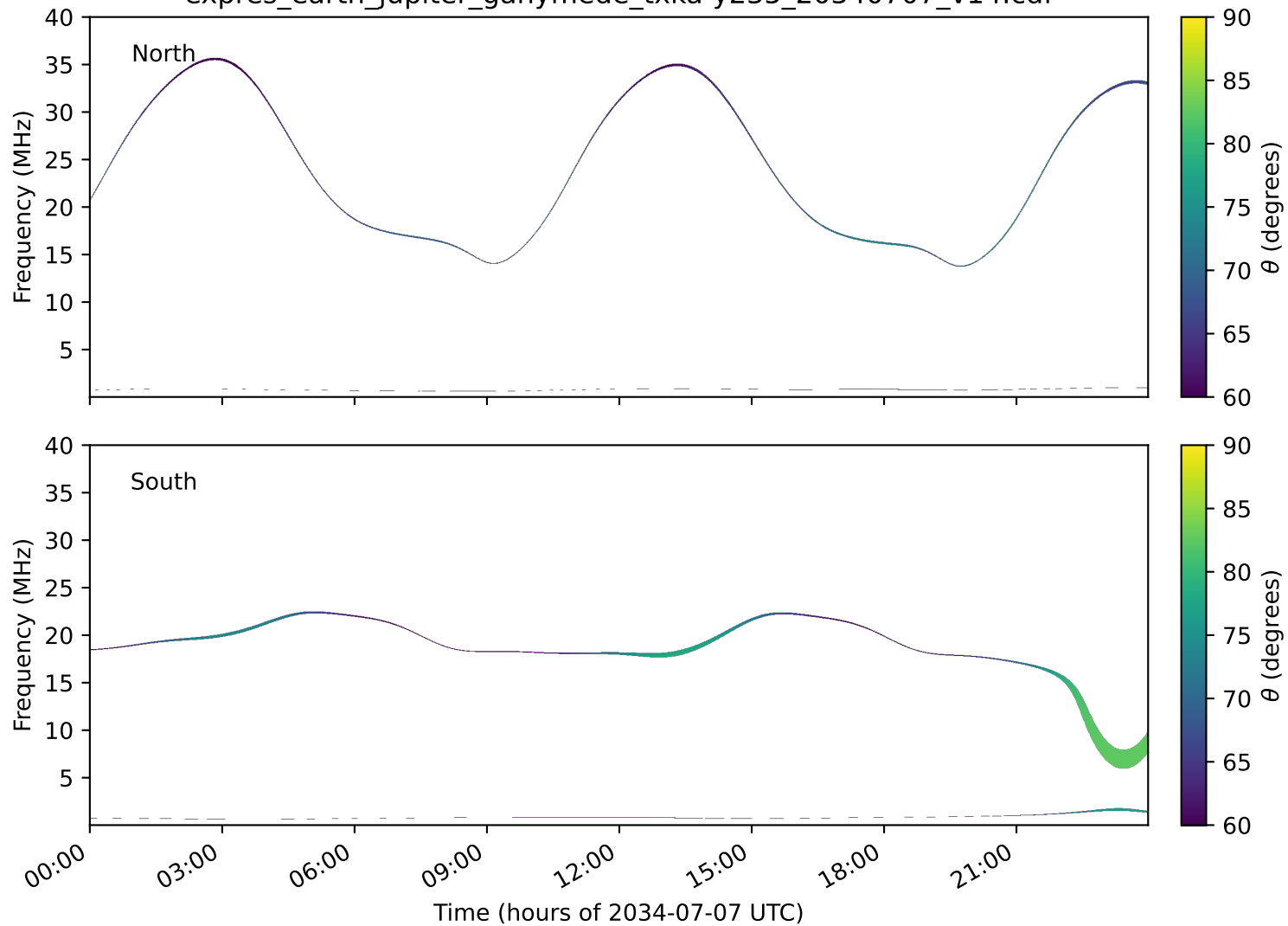
expres_earth_jupiter_ganymede_txka-y235_20340707_v14.cdf
