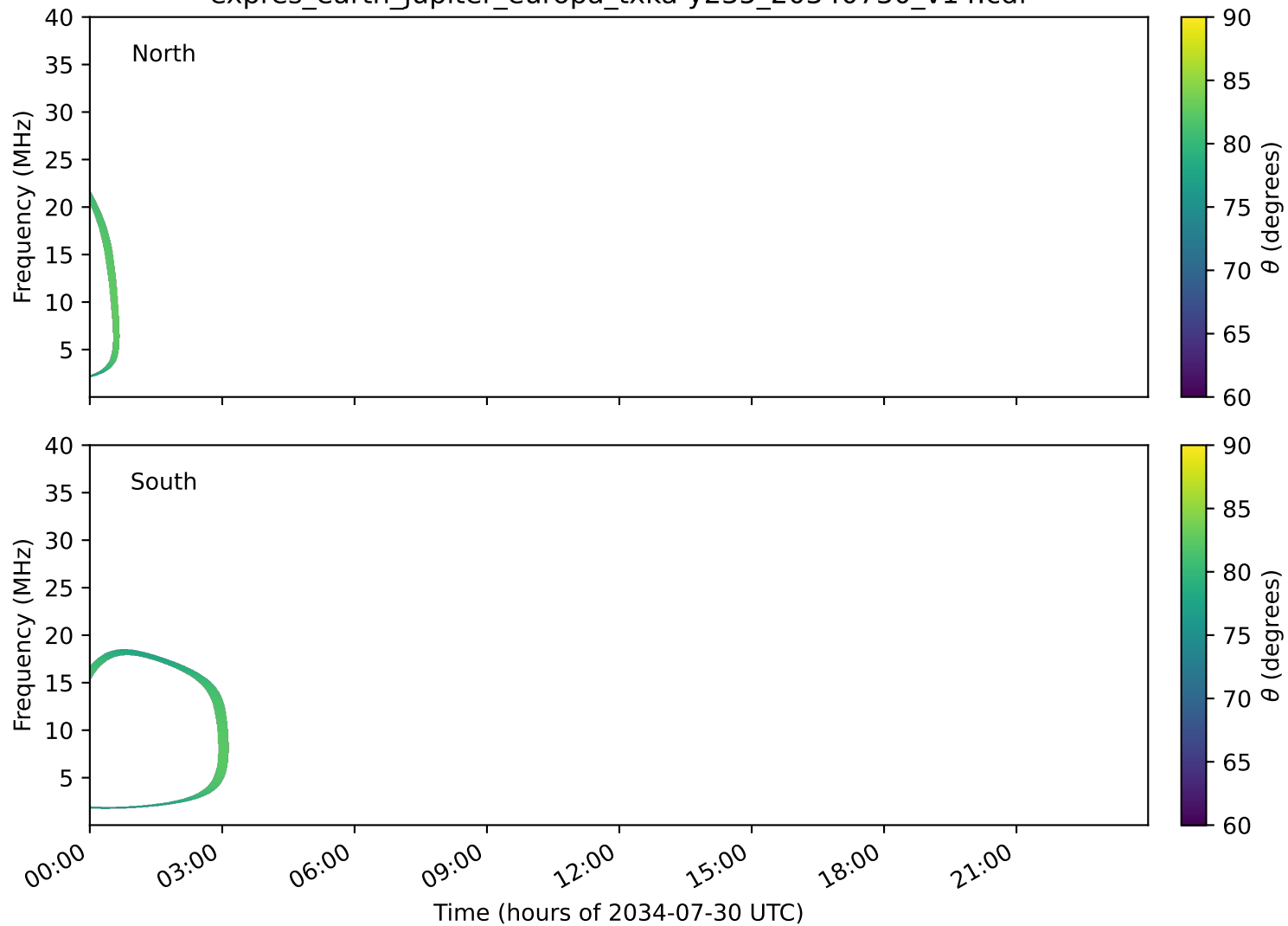
expres_earth_jupiter_europa_txka-y235_20340730_v14.cdf
