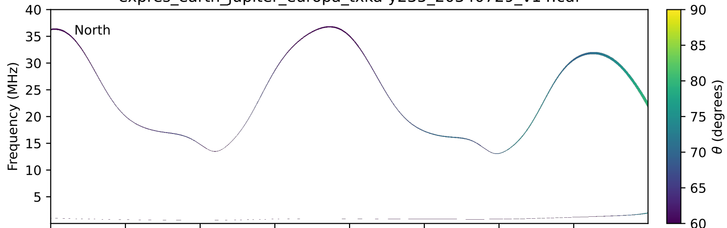
expres_earth_jupiter_europa_txka-y235_20340729_v14.cdf
