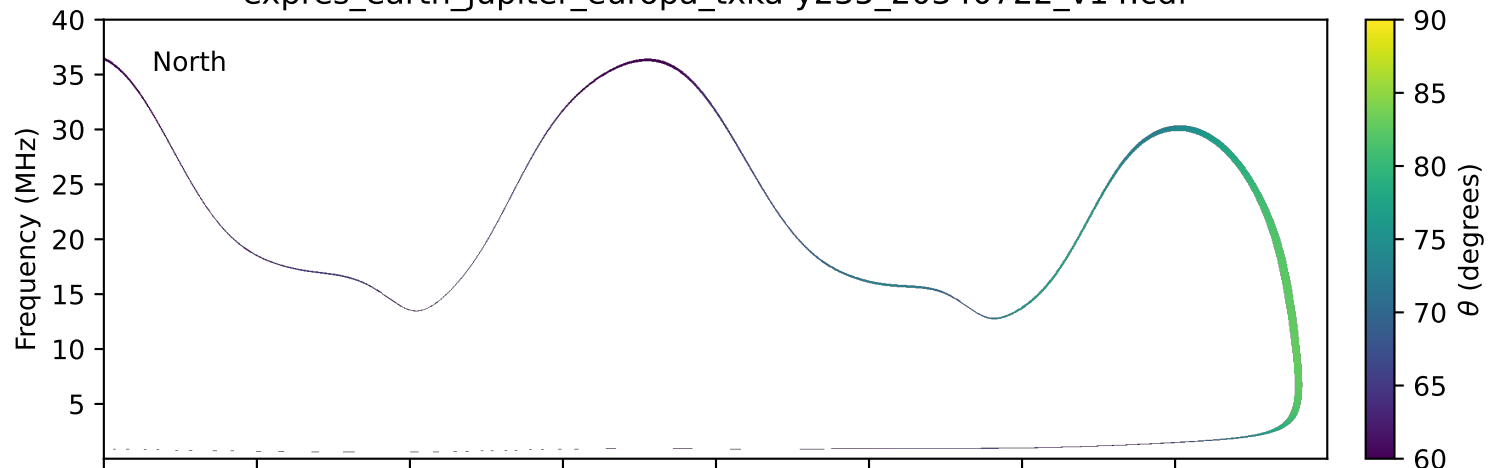
expres_earth_jupiter_europa_txka-y235_20340722_v14.cdf
