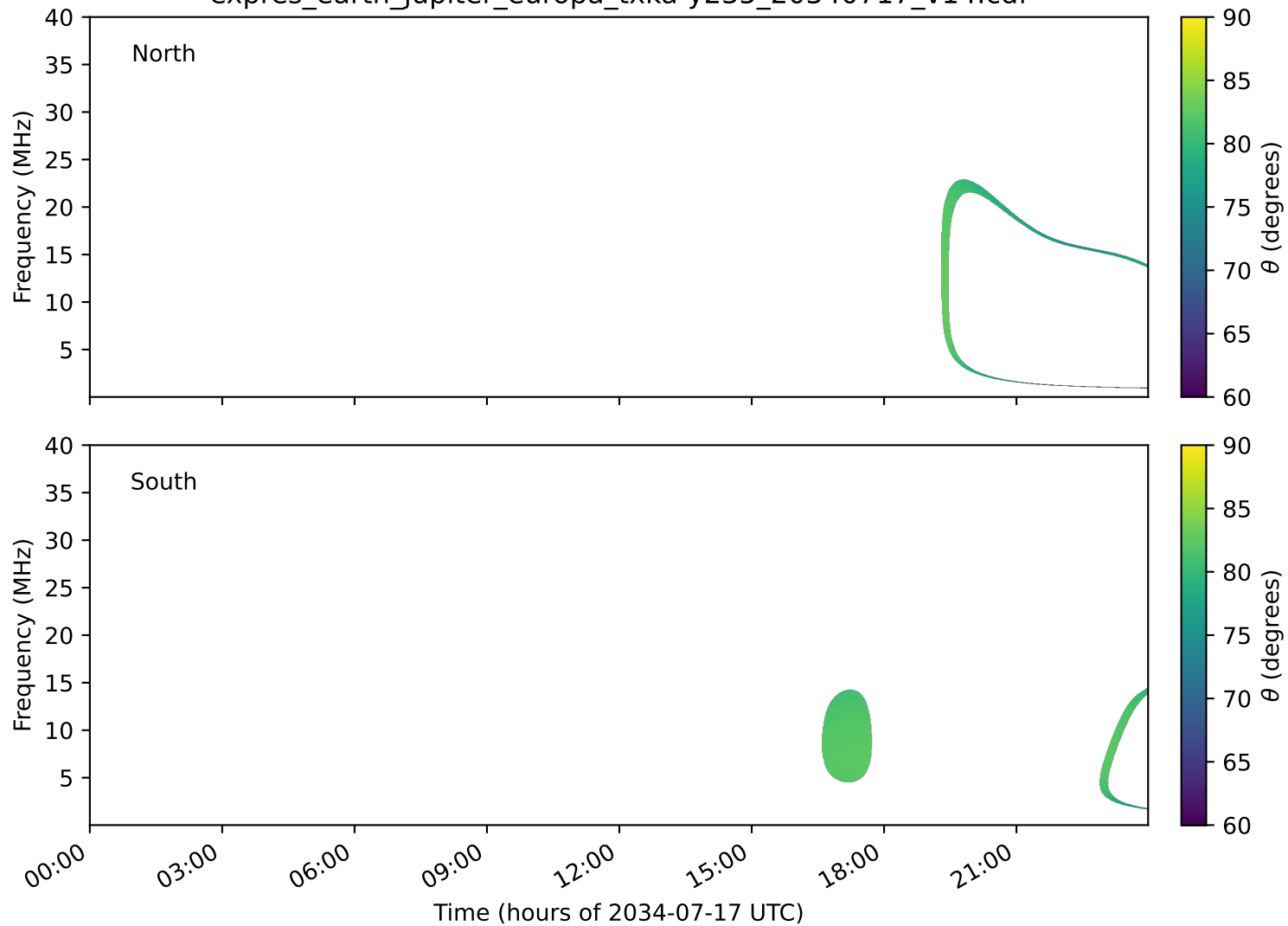
expres_earth_jupiter_europa_txka-y235_20340717_v14.cdf
