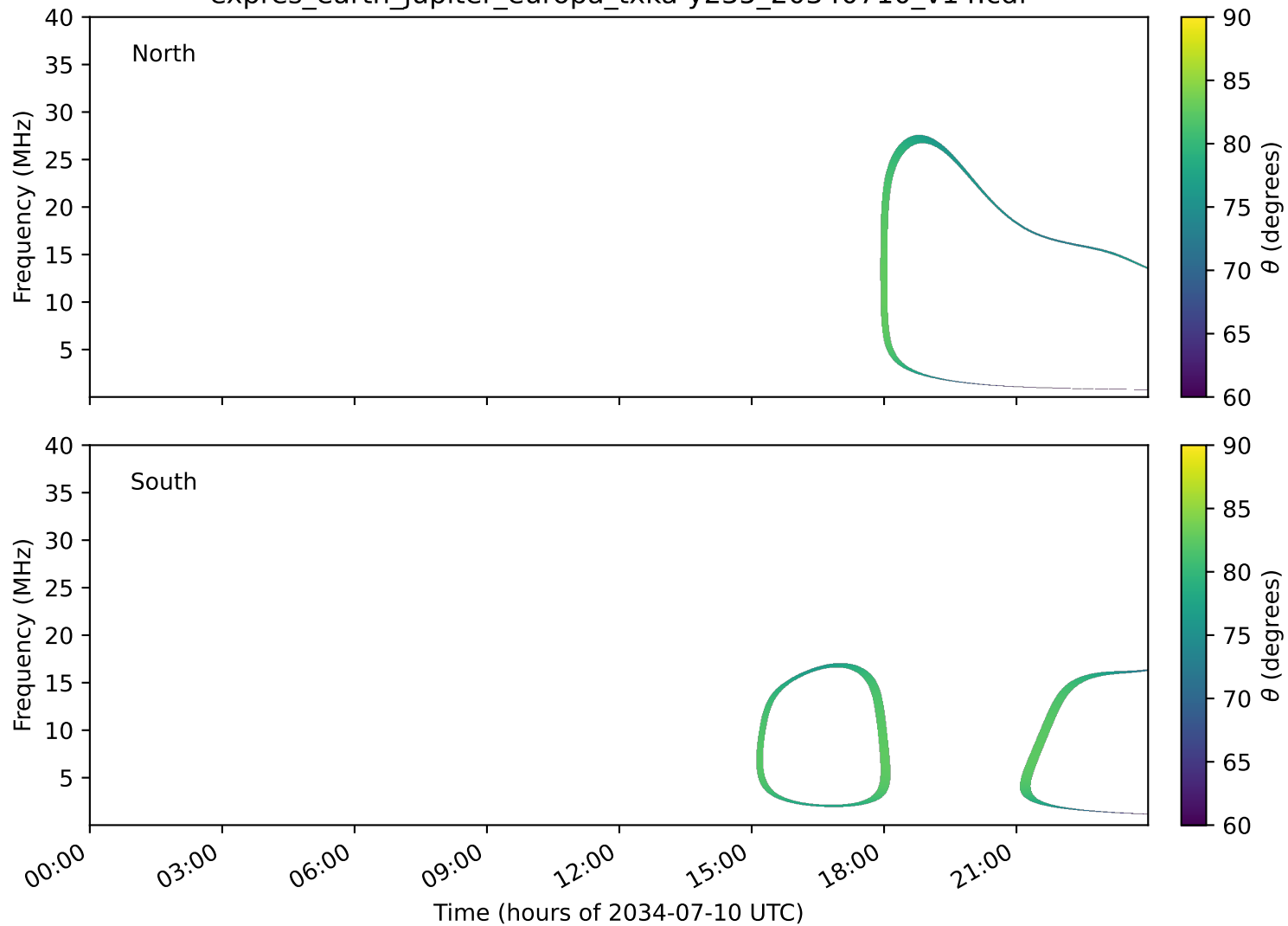
expres_earth_jupiter_europa_txka-y235_20340710_v14.cdf
