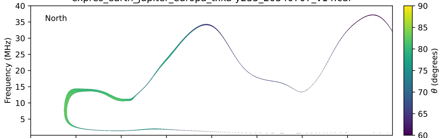
expres_earth_jupiter_europa_txka-y235_20340707_v14.cdf
