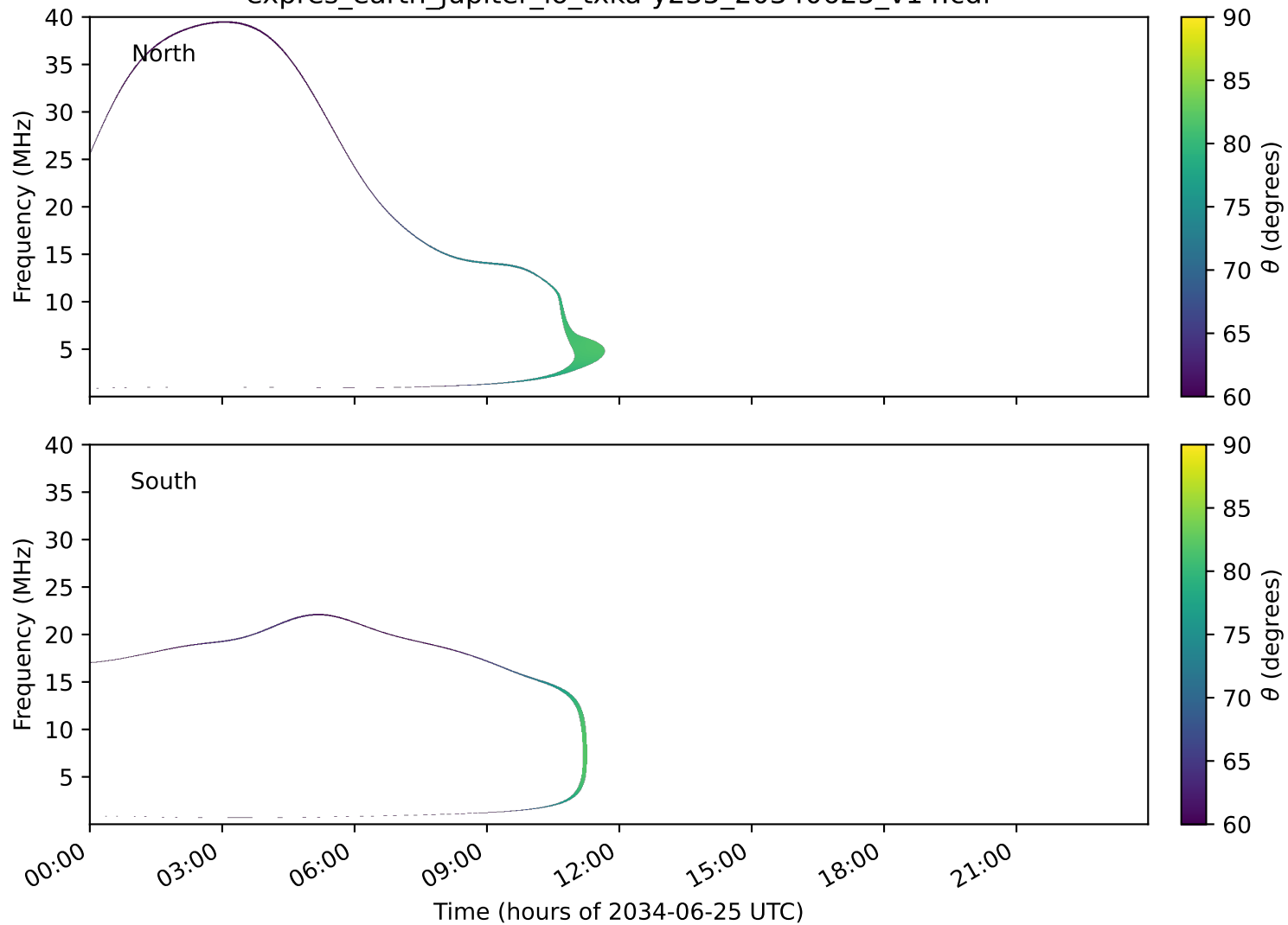
expres_earth_jupiter_io_txka-y235_20340625_v14.cdf
