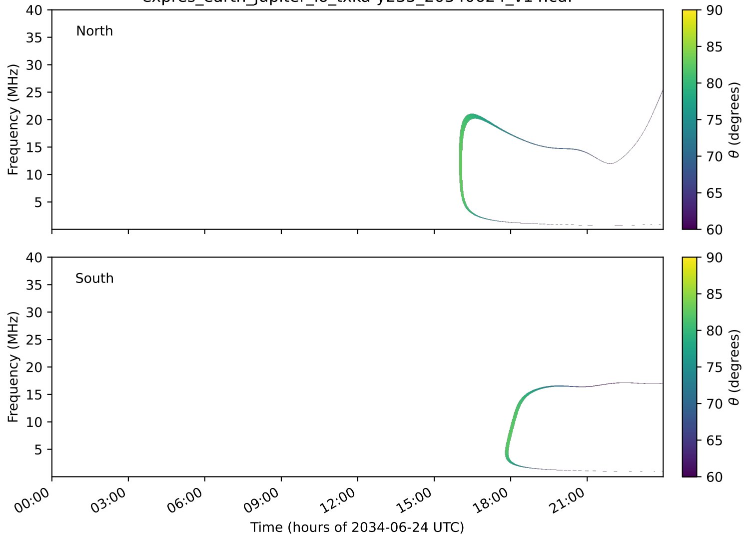
expres_earth_jupiter_io_txka-y235_20340624_v14.cdf
