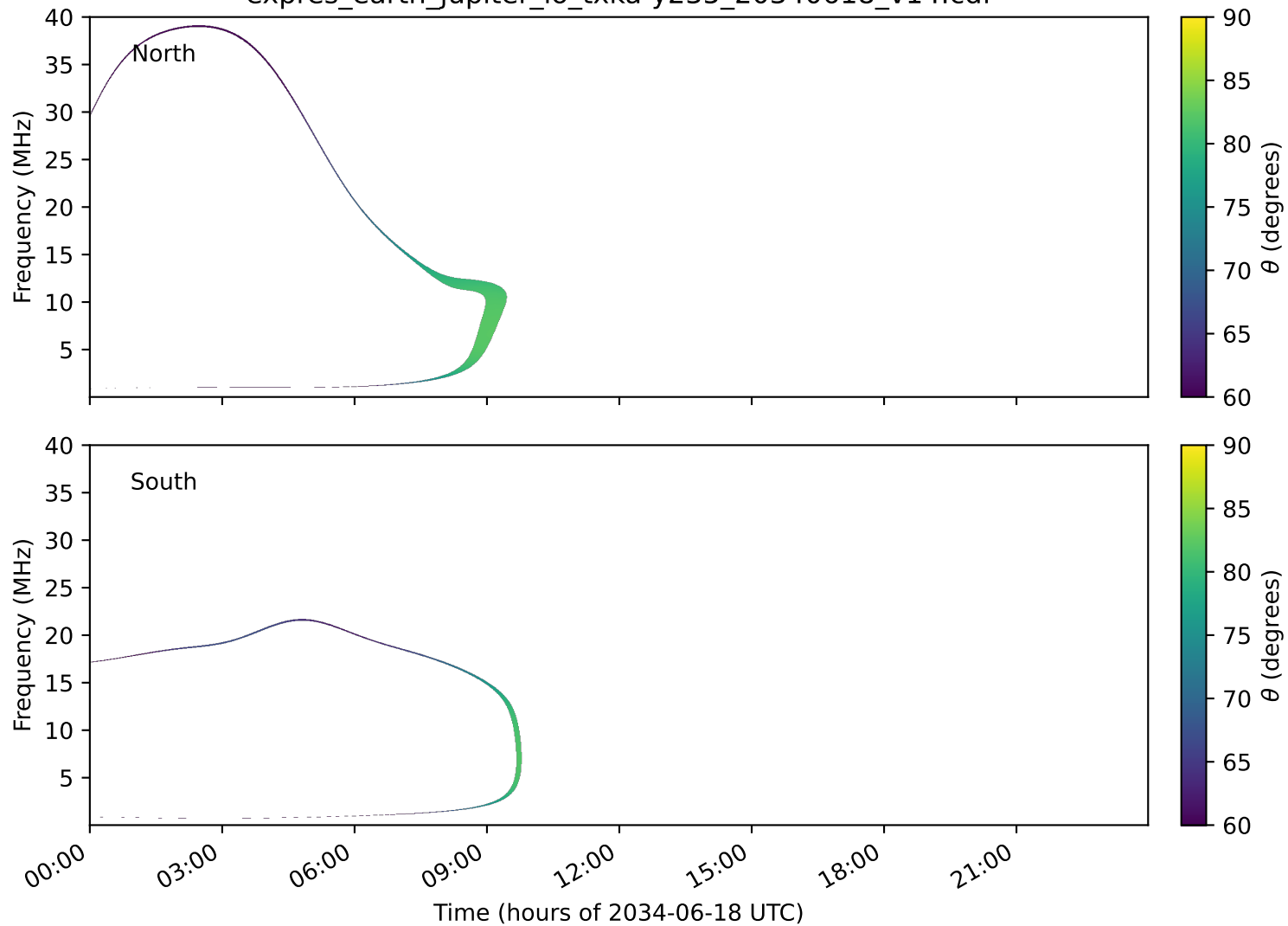
expres_earth_jupiter_io_txka-y235_20340618_v14.cdf
