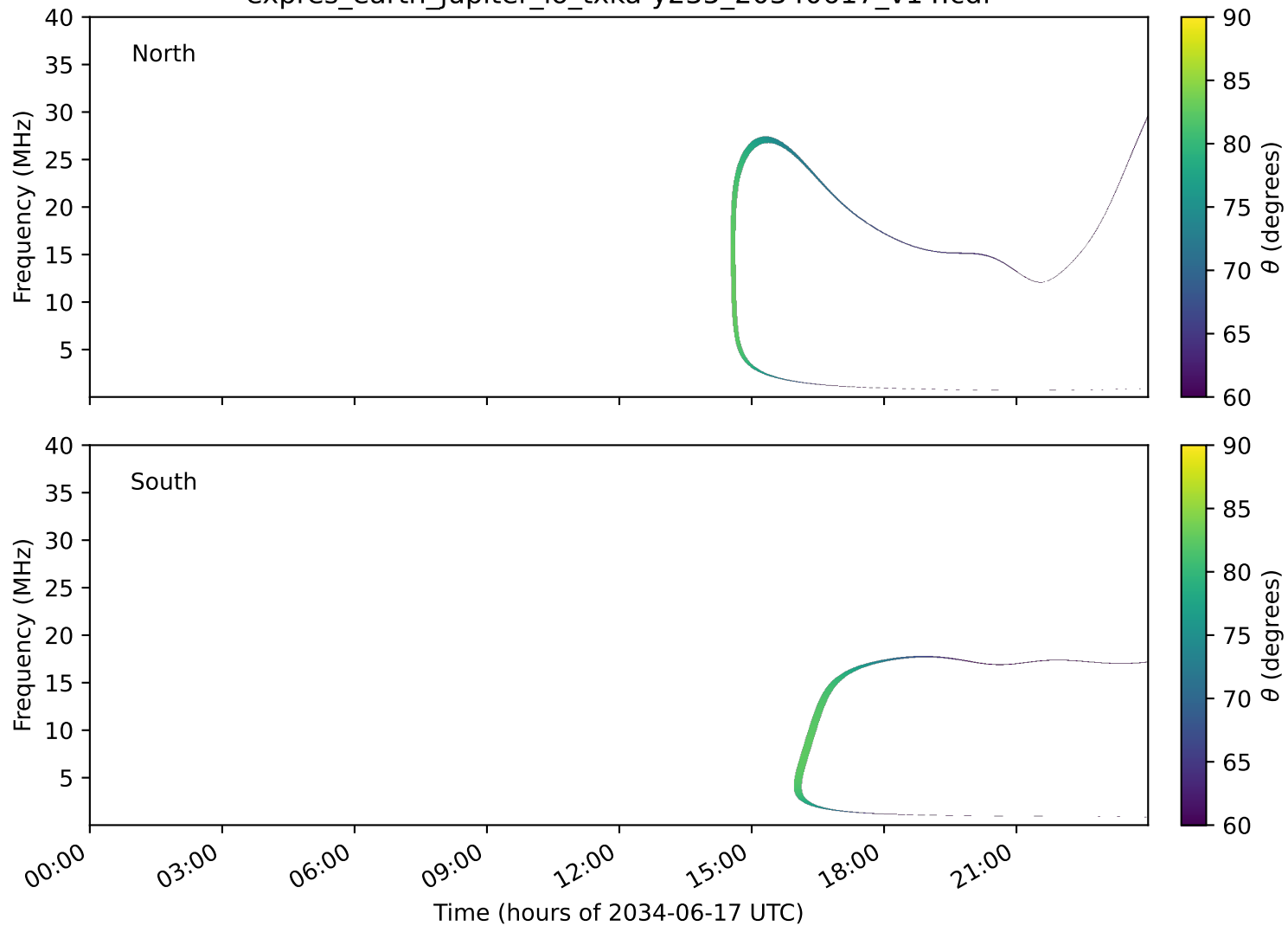
expres_earth_jupiter_io_txka-y235_20340617_v14.cdf
