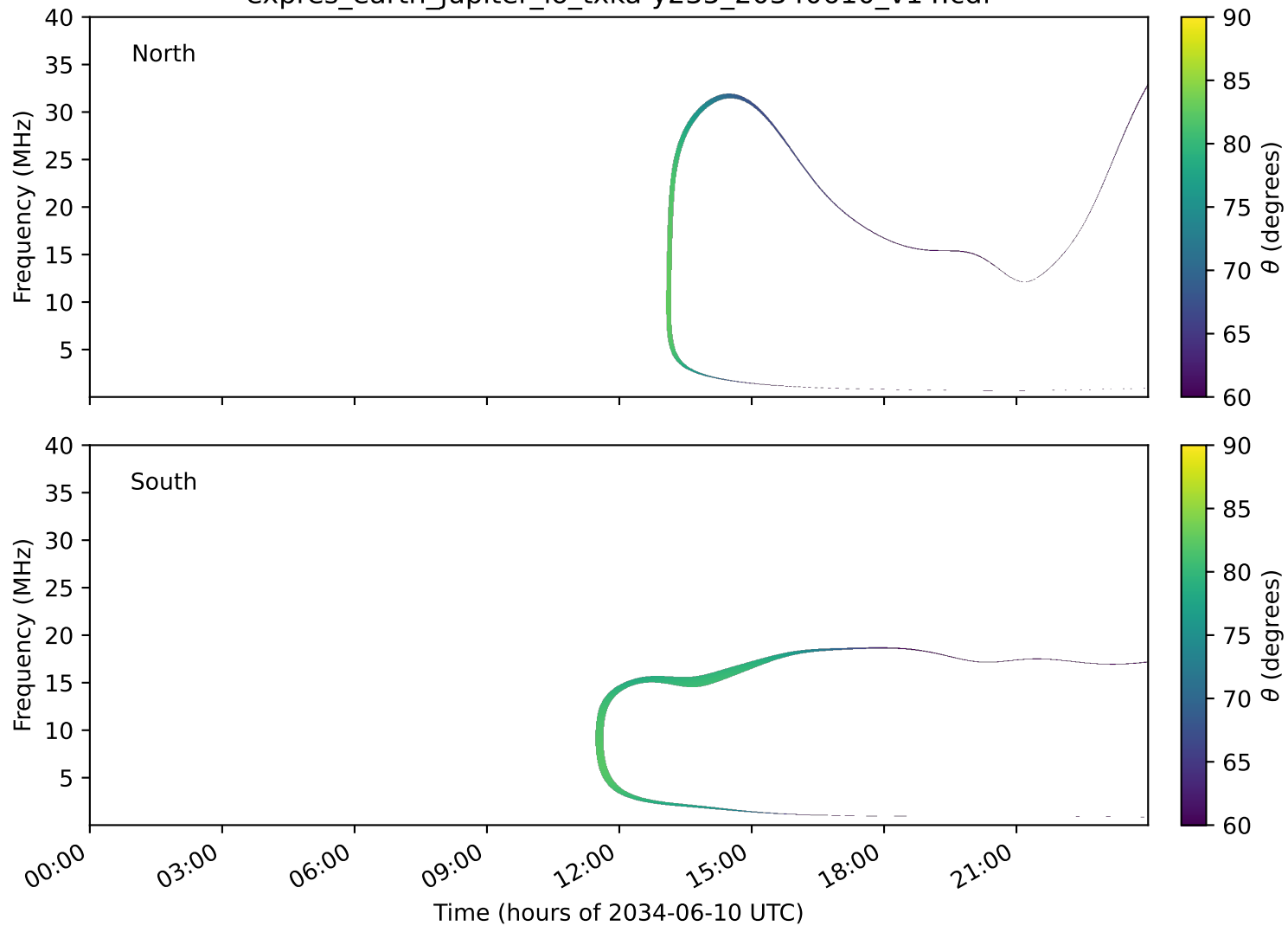
expres_earth_jupiter_io_txka-y235_20340610_v14.cdf
