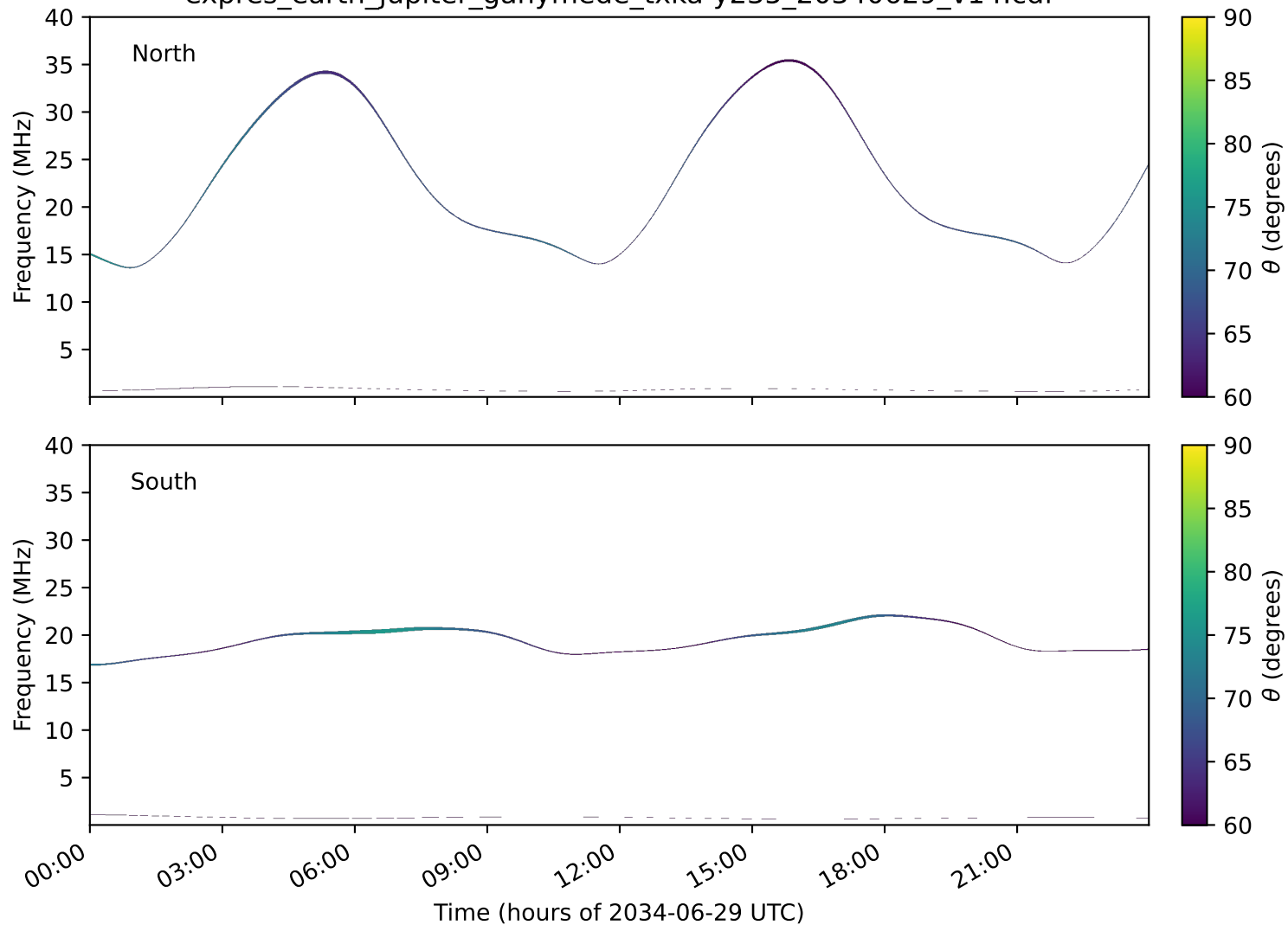
expres_earth_jupiter_ganymede_txka-y235_20340629_v14.cdf
