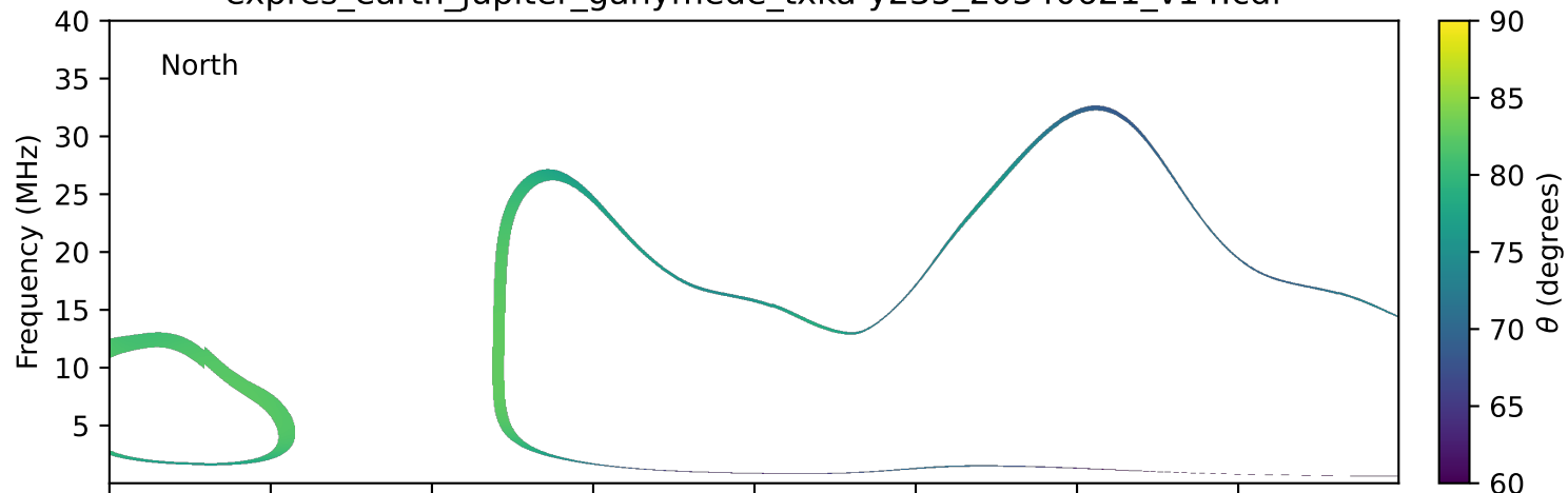
expres_earth_jupiter_ganymede_txka-y235_20340621_v14.cdf
