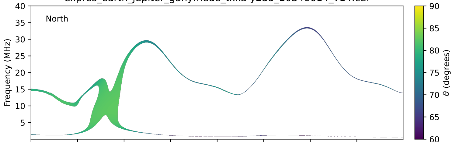
expres_earth_jupiter_ganymede_txka-y235_20340614_v14.cdf
