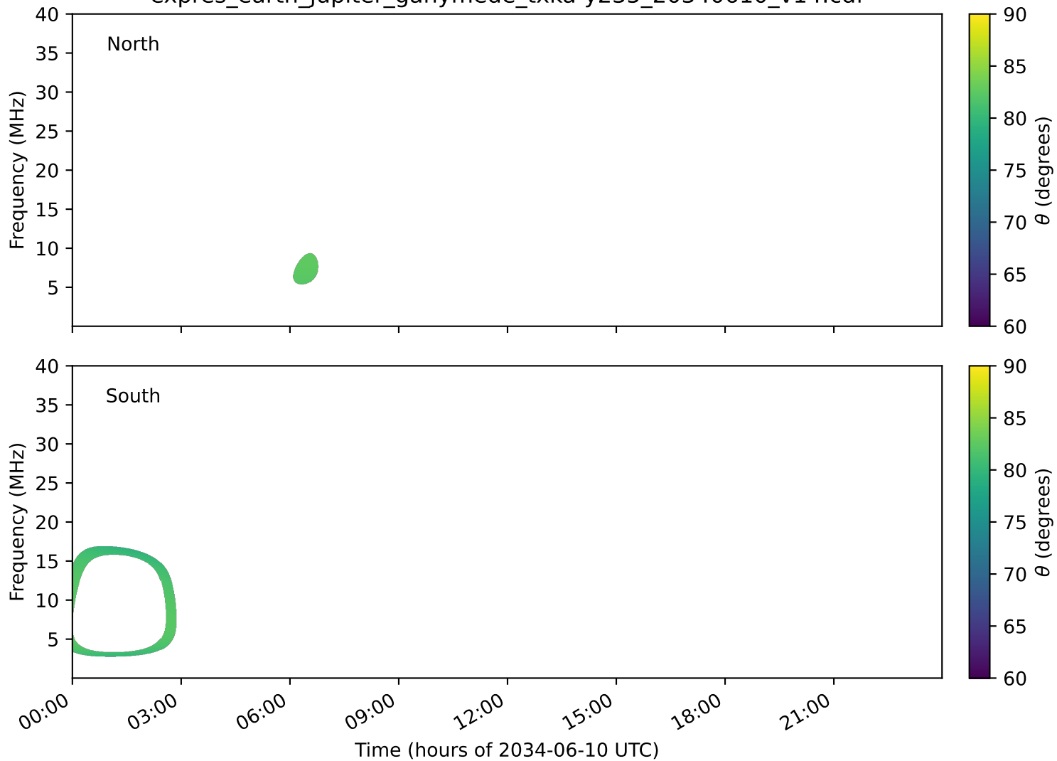
expres_earth_jupiter_ganymede_txka-y235_20340610_v14.cdf
