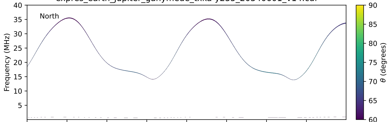
expres_earth_jupiter_ganymede_txka-y235_20340601_v14.cdf
