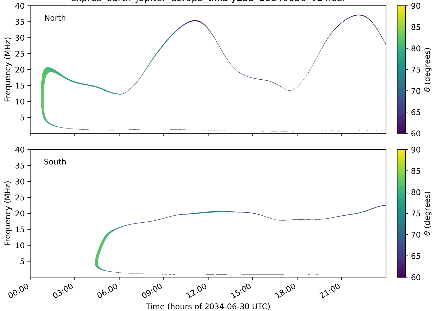
expres_earth_jupiter_europa_txka-y235_20340630_v14.cdf
