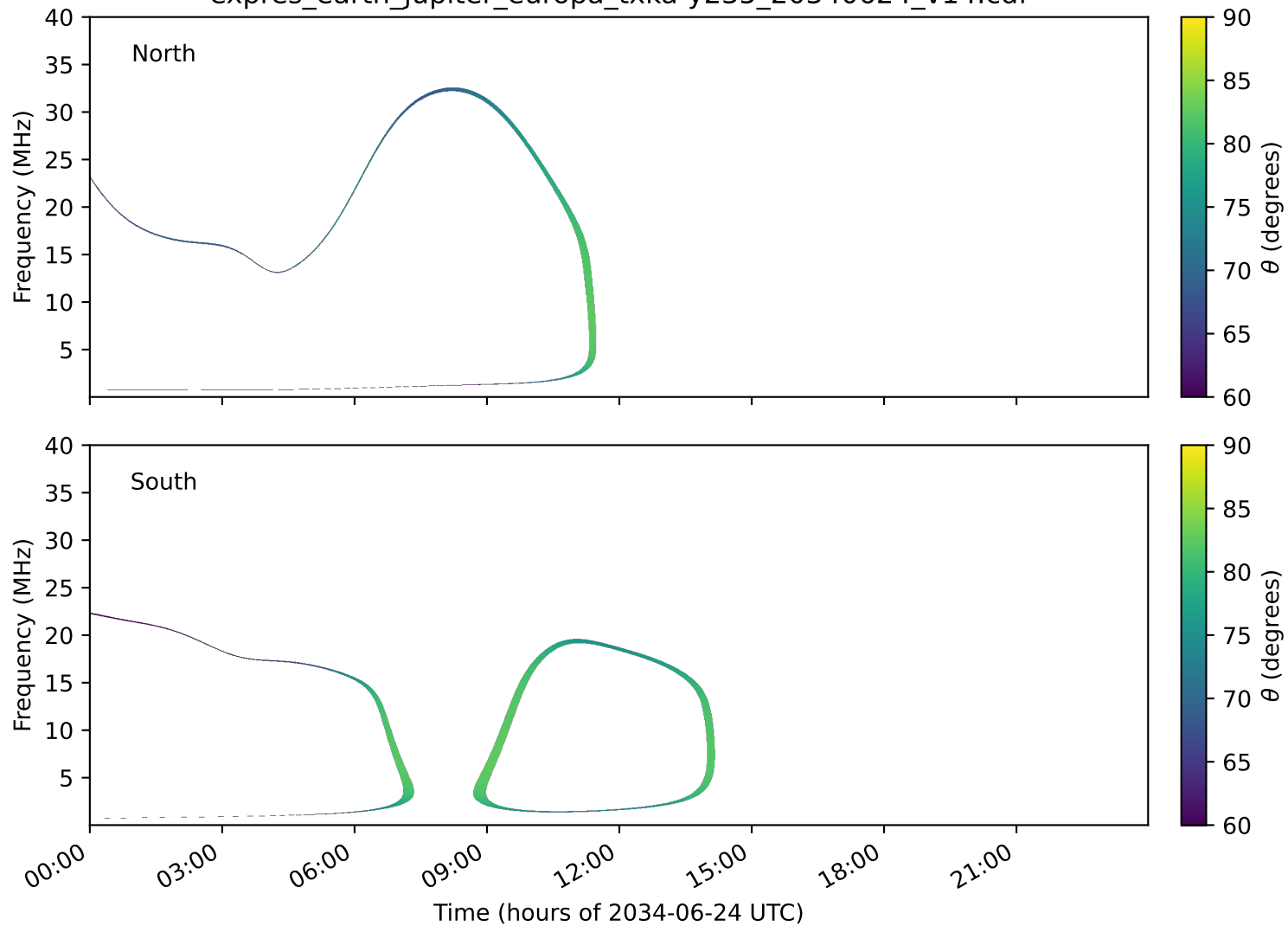
expres_earth_jupiter_europa_txka-y235_20340624_v14.cdf
