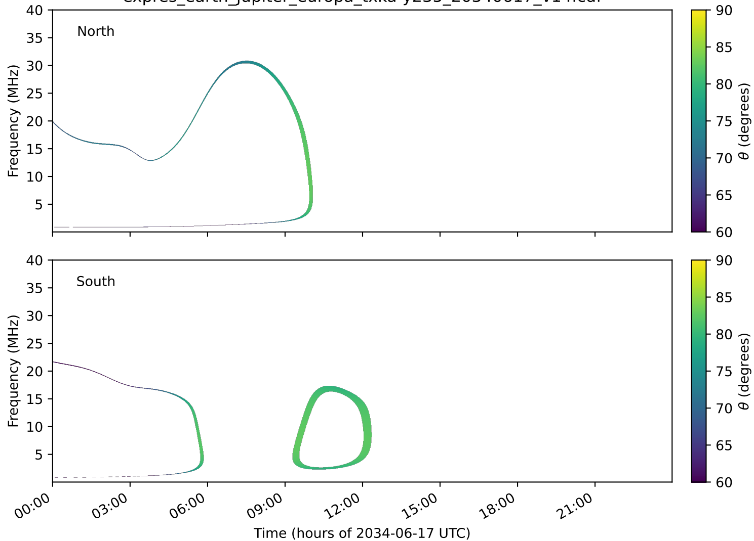
expres_earth_jupiter_europa_txka-y235_20340617_v14.cdf
