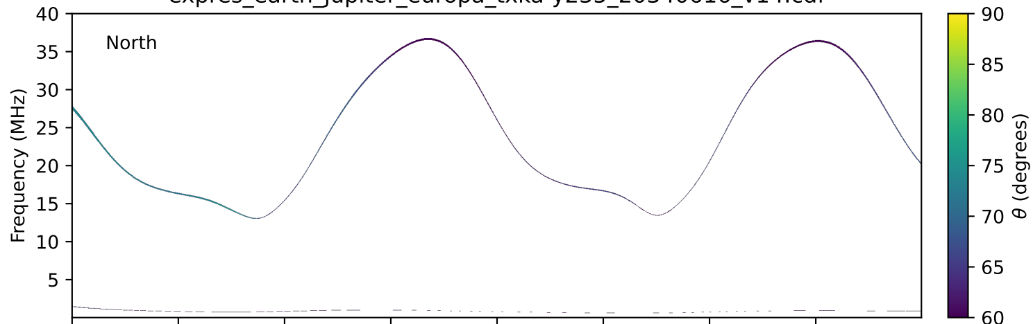
expres_earth_jupiter_europa_txka-y235_20340616_v14.cdf
