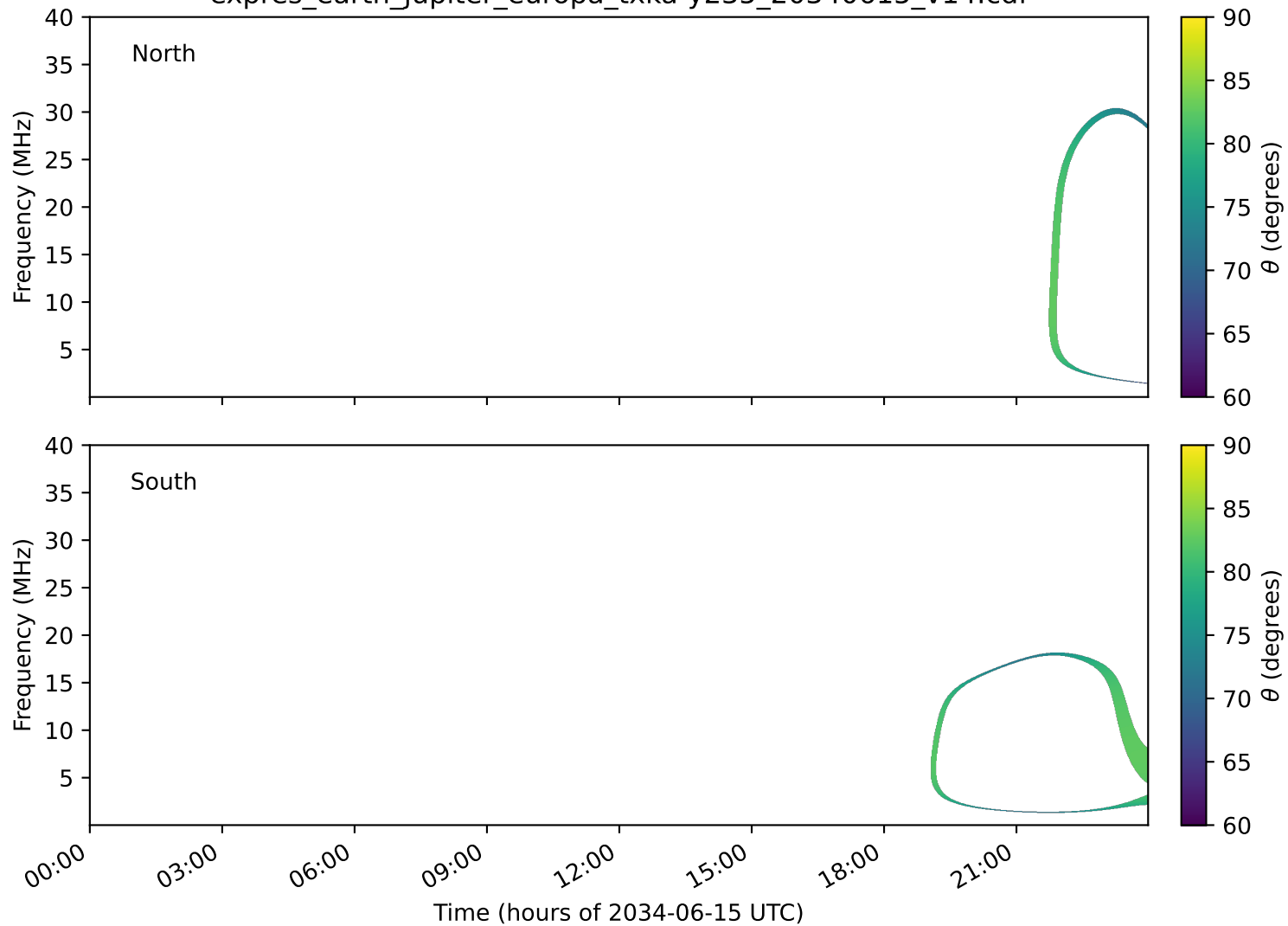
expres_earth_jupiter_europa_txka-y235_20340615_v14.cdf
