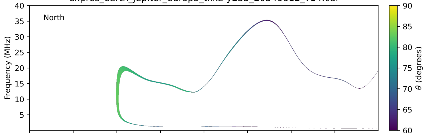
expres_earth_jupiter_europa_txka-y235_20340612_v14.cdf
