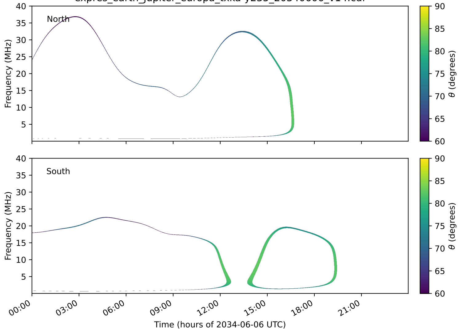
expres_earth_jupiter_europa_txka-y235_20340606_v14.cdf
