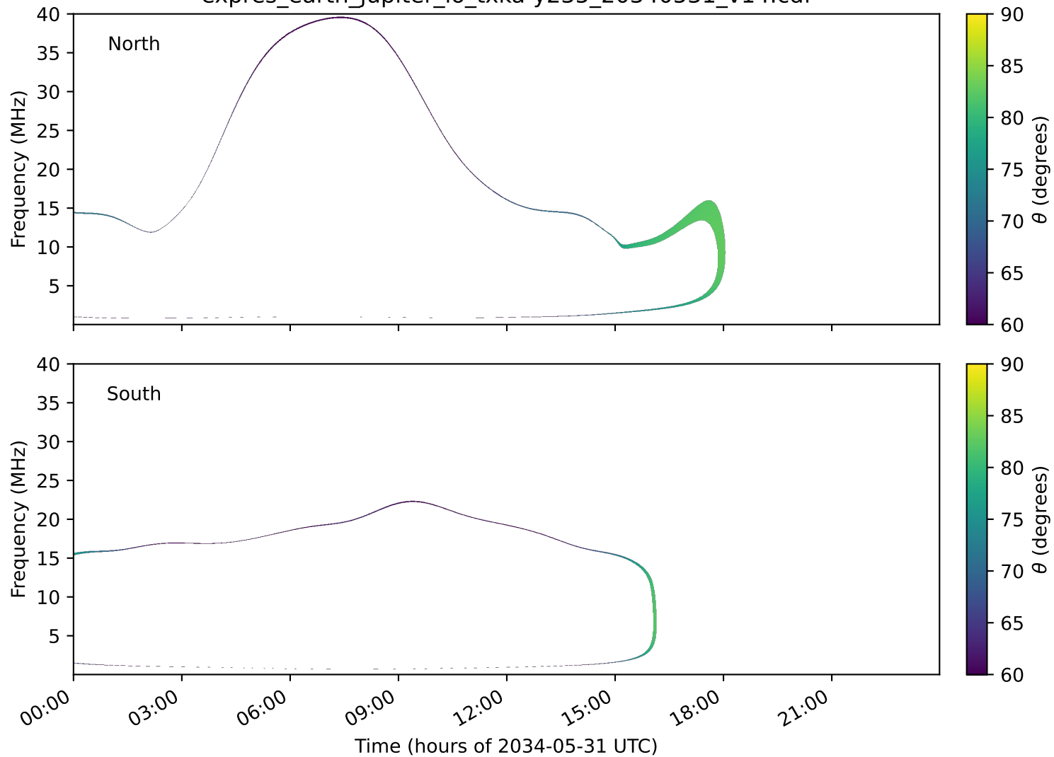
expres_earth_jupiter_io_txka-y235_20340531_v14.cdf
