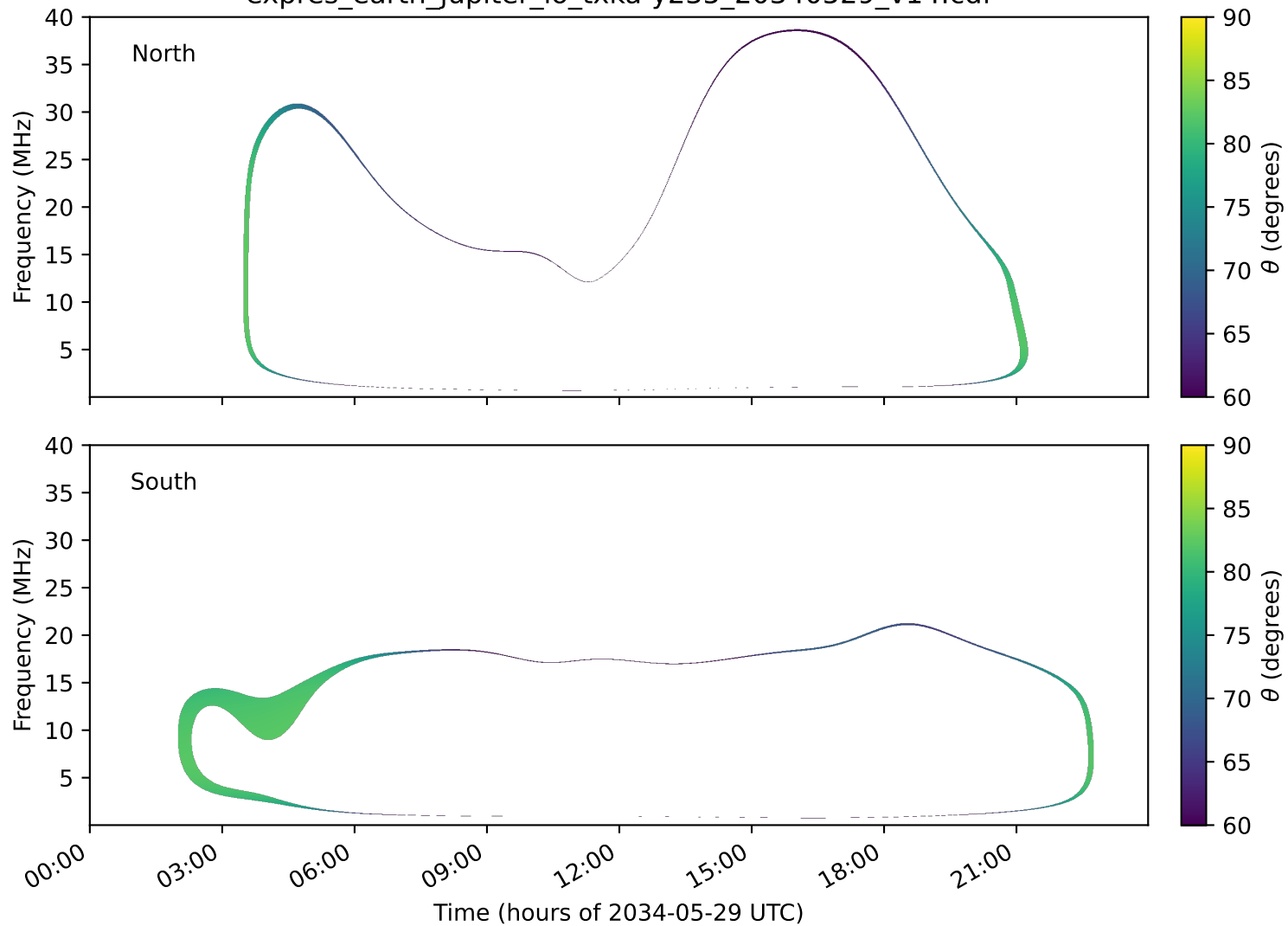
expres_earth_jupiter_io_txka-y235_20340529_v14.cdf
