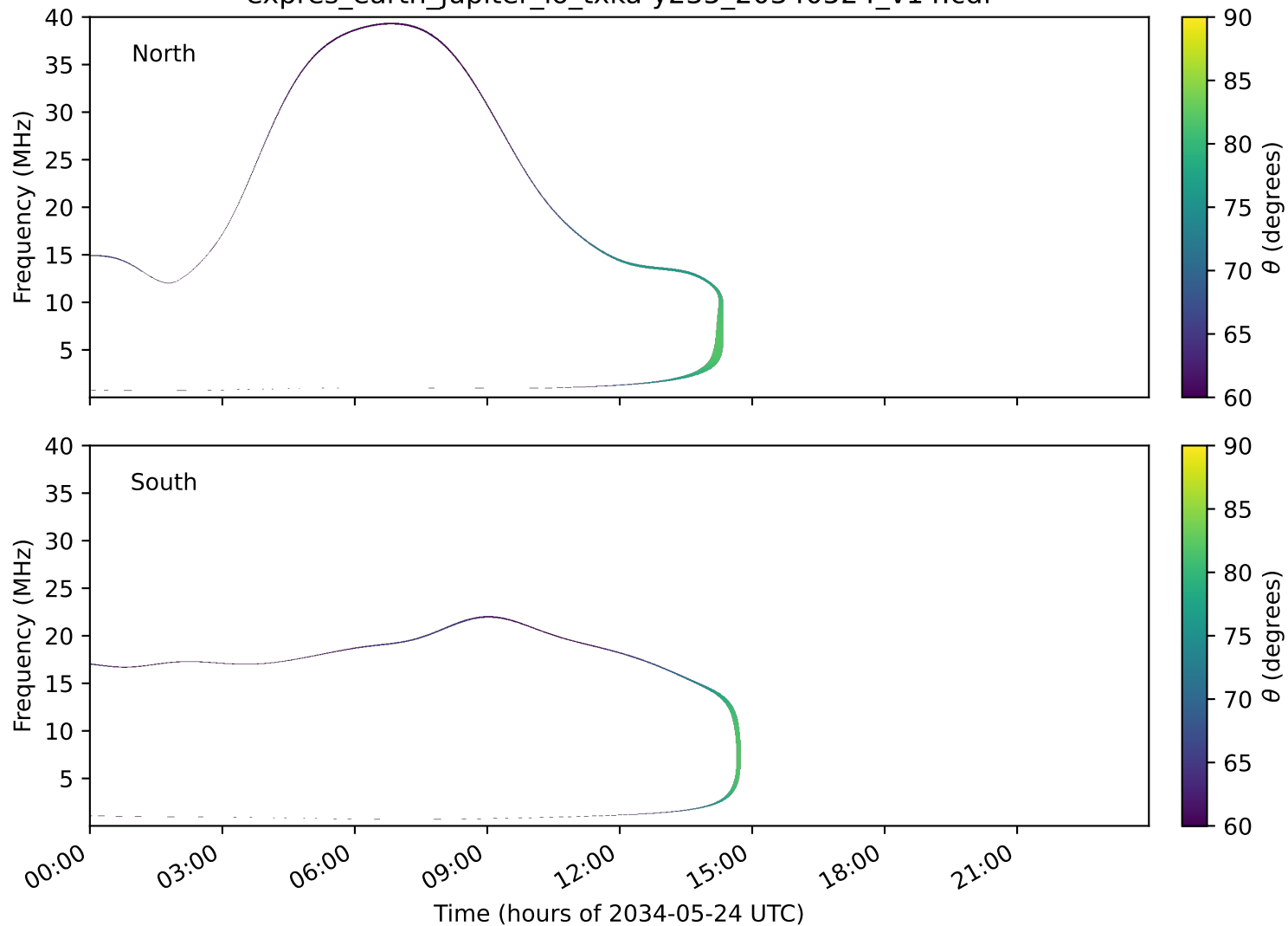
expres_earth_jupiter_io_txka-y235_20340524_v14.cdf
