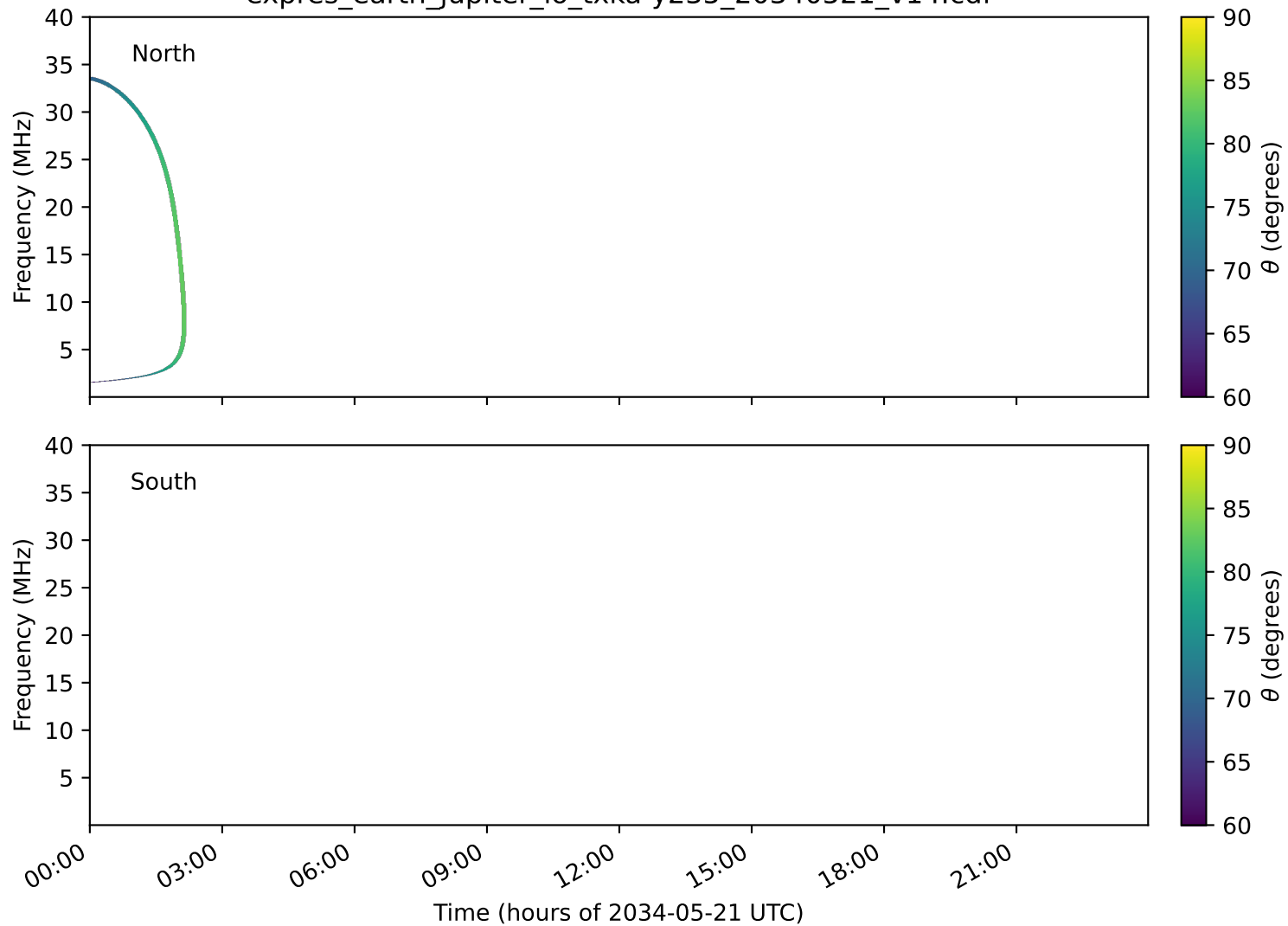
expres_earth_jupiter_io_txka-y235_20340521_v14.cdf
