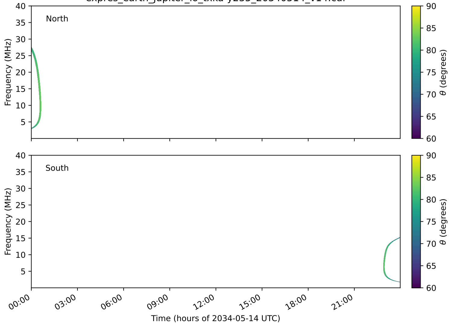
expres_earth_jupiter_io_txka-y235_20340514_v14.cdf
