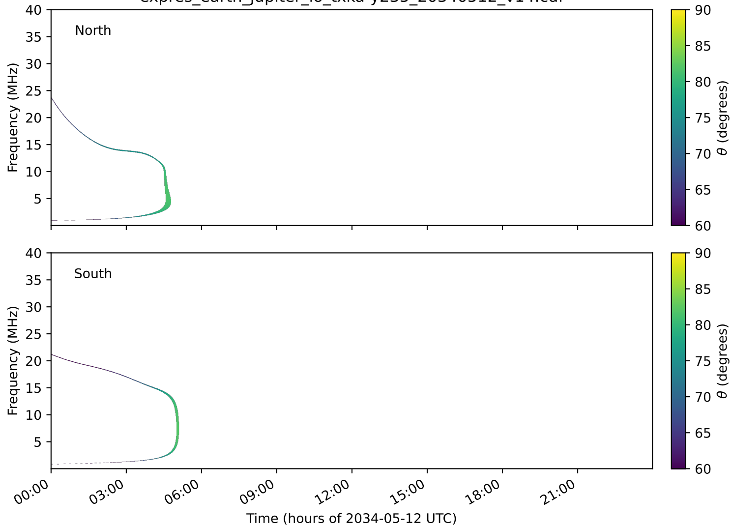
expres_earth_jupiter_io_txka-y235_20340512_v14.cdf
