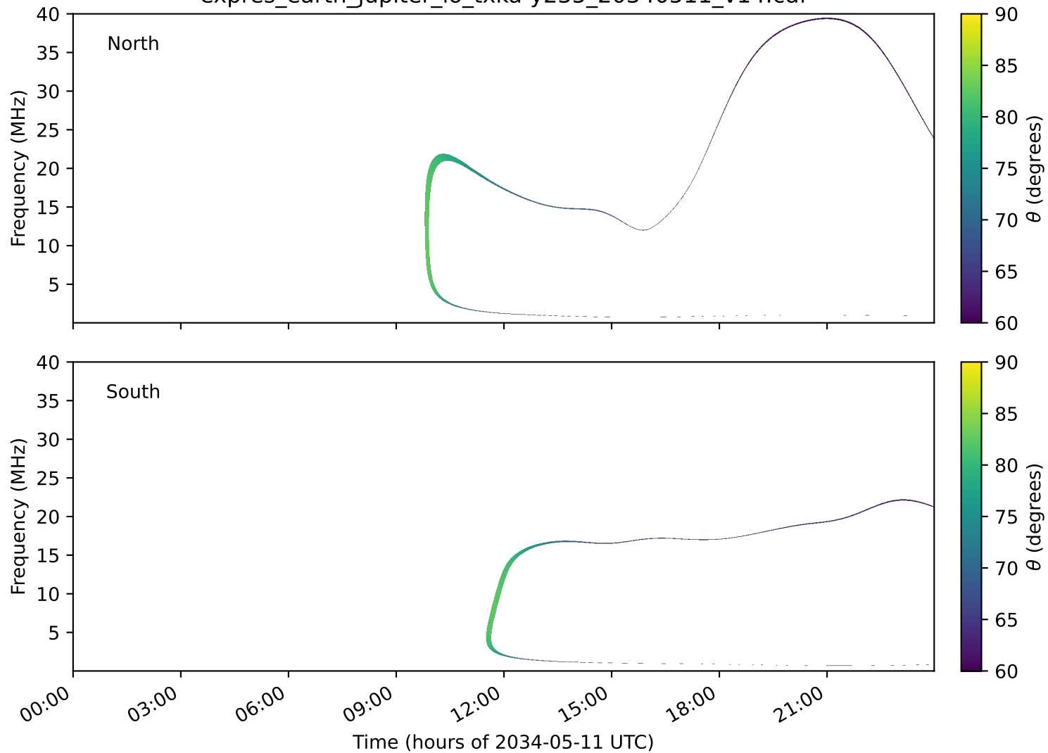
expres_earth_jupiter_io_txka-y235_20340511_v14.cdf
