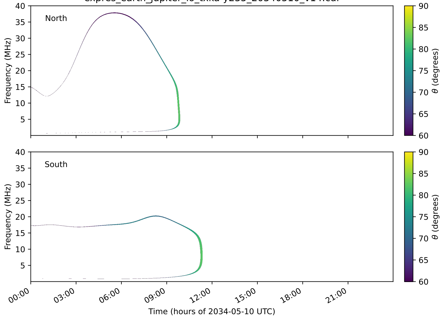
expres_earth_jupiter_io_txka-y235_20340510_v14.cdf
