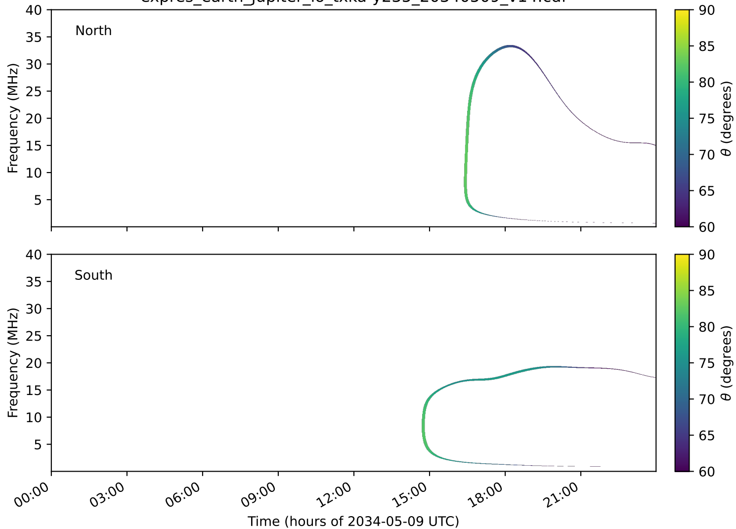
expres_earth_jupiter_io_txka-y235_20340509_v14.cdf
