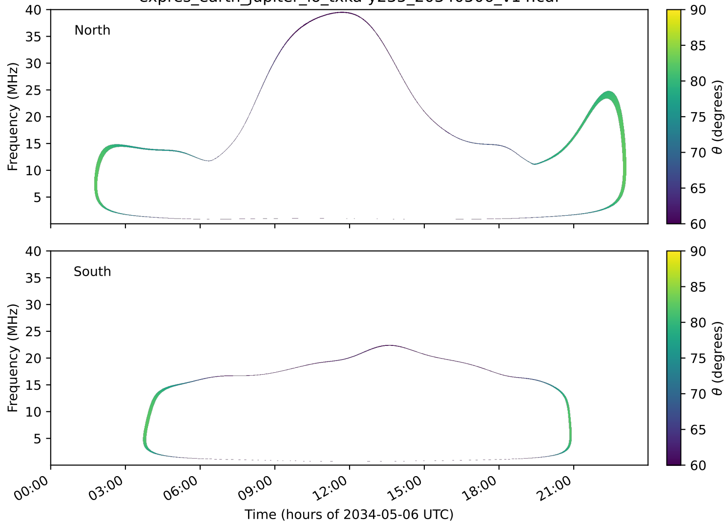
expres_earth_jupiter_io_txka-y235_20340506_v14.cdf
