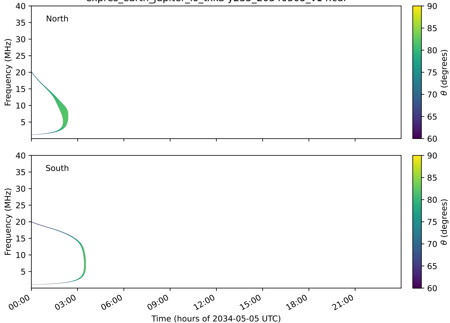
expres_earth_jupiter_io_txka-y235_20340505_v14.cdf
