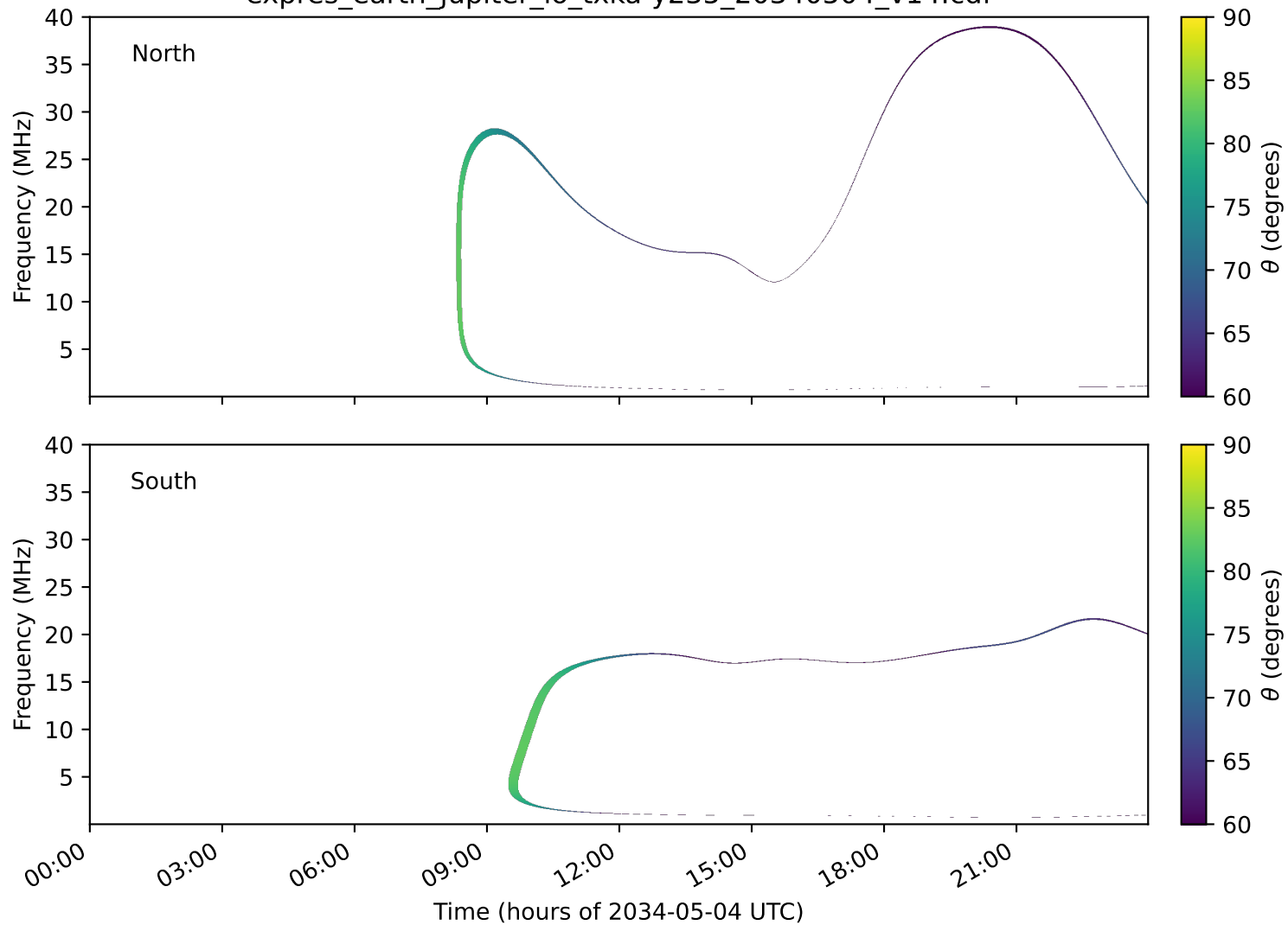
expres_earth_jupiter_io_txka-y235_20340504_v14.cdf
