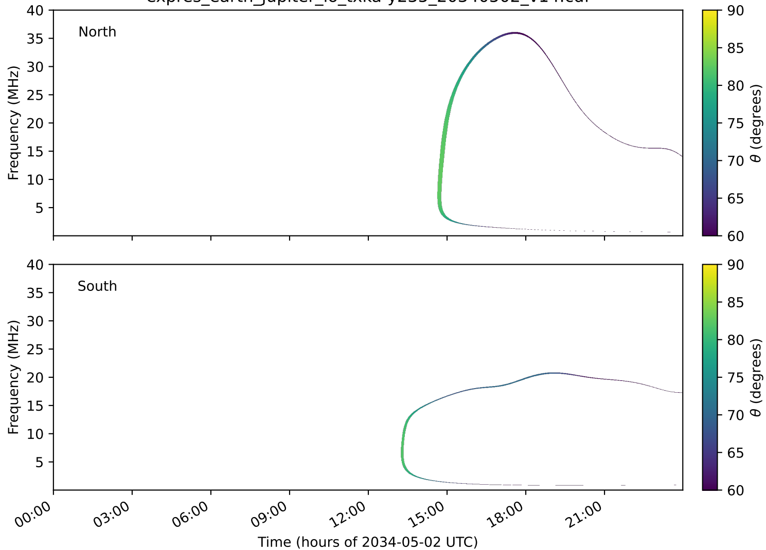
expres_earth_jupiter_io_txka-y235_20340502_v14.cdf
