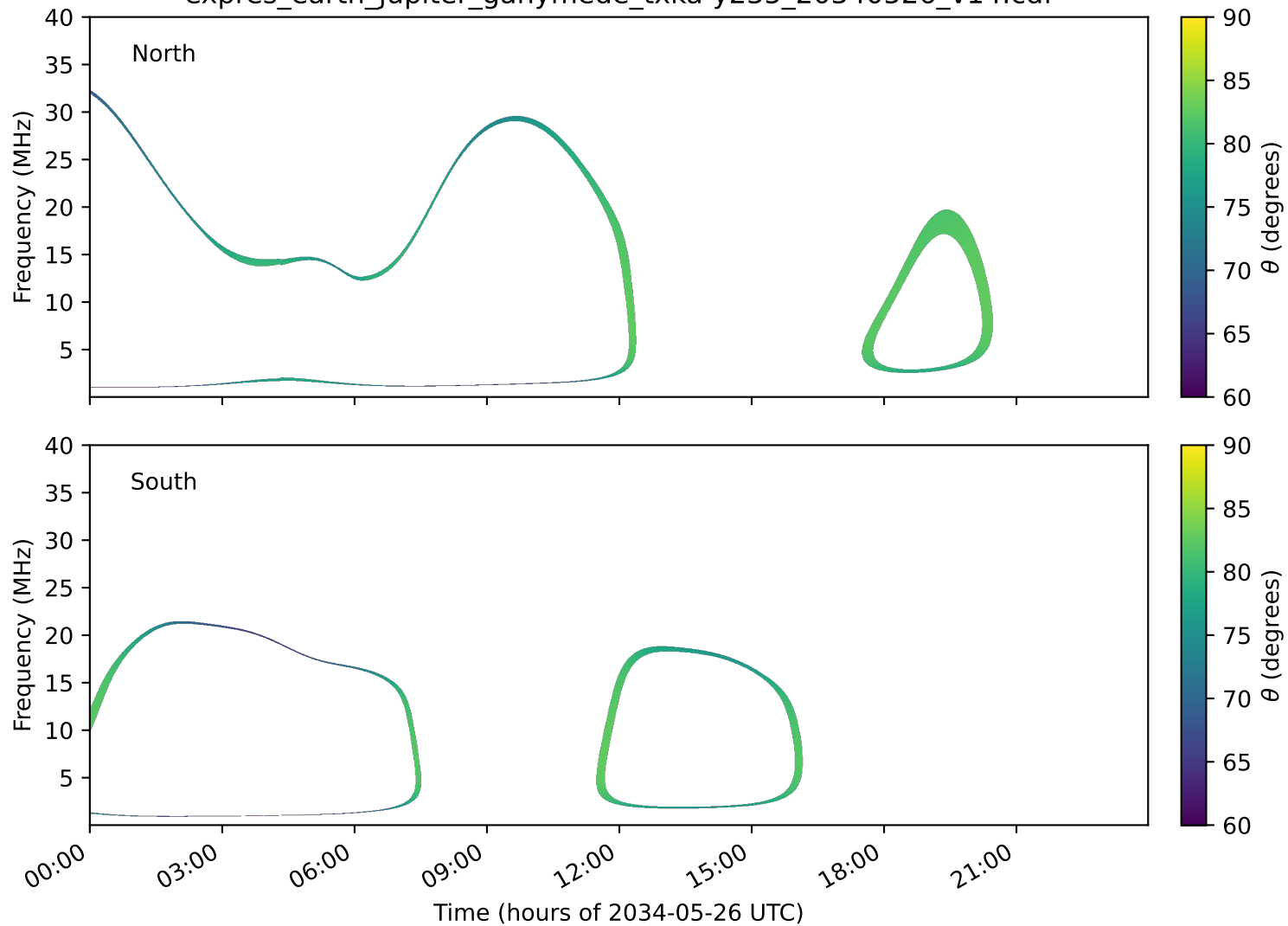
expres_earth_jupiter_ganymede_txka-y235_20340526_v14.cdf
